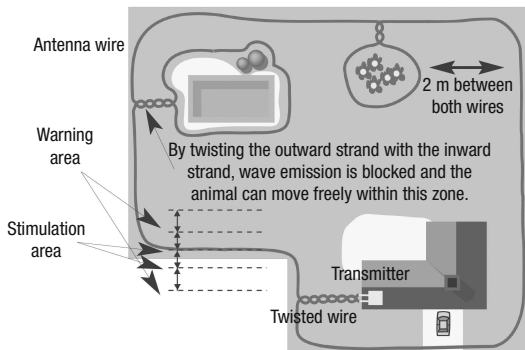
Diagram 3 – Sample installation
